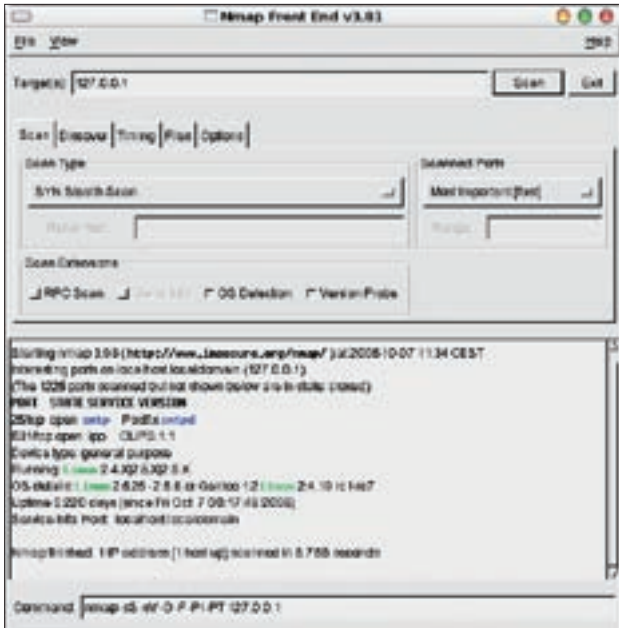
Figure 1: The Nmap front-end removes the need to learn the enormous range of options, and gives the administrator a ready-to-run command line (see the bottom of the figure.)
