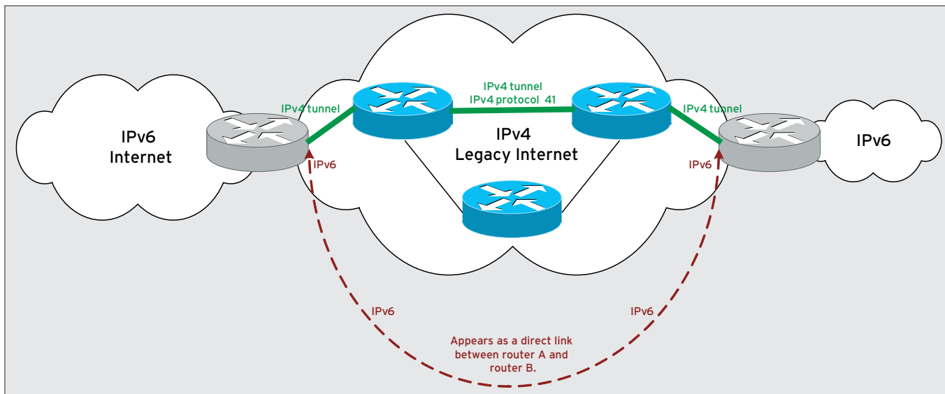
Figure 4: Tunnel brokers provide tunneled access to an IPv6 network via IPv4.
